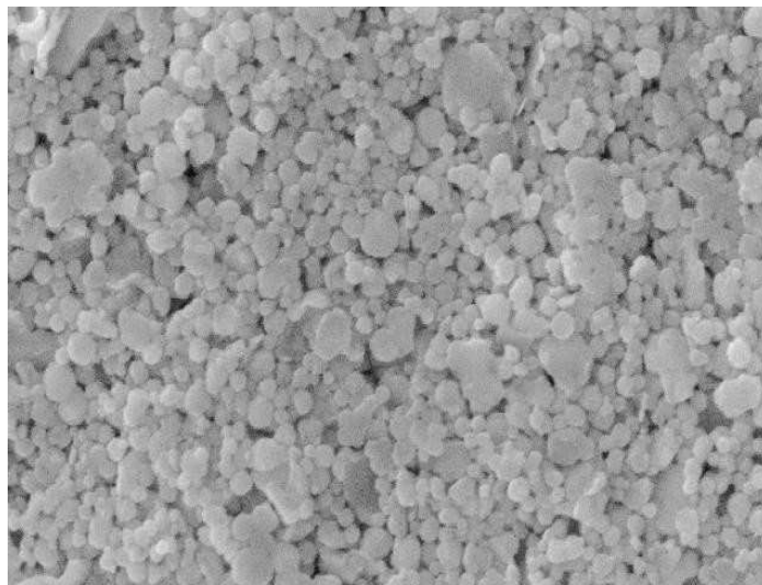
10kx SEM of 90%/10% Pd AgPd 7590PA
