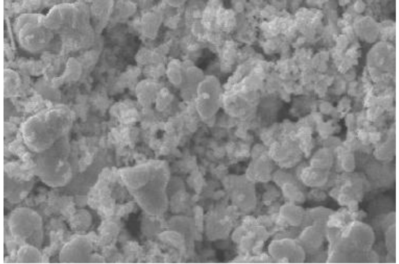
5kx SEM of 100% Pd 7660 Powder
