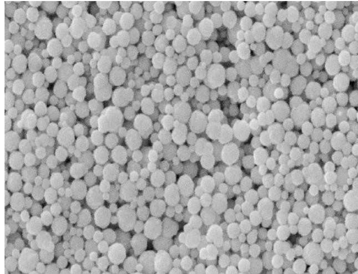
10kx SEM of 70% Ag/ 30% Pd 7011
